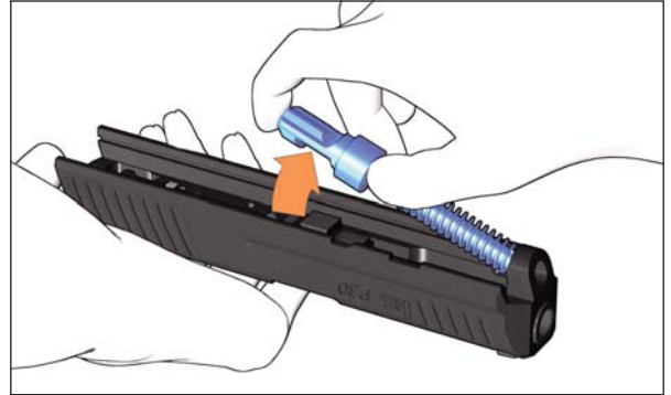
Fig. 41a: Pull slide back and lock it
